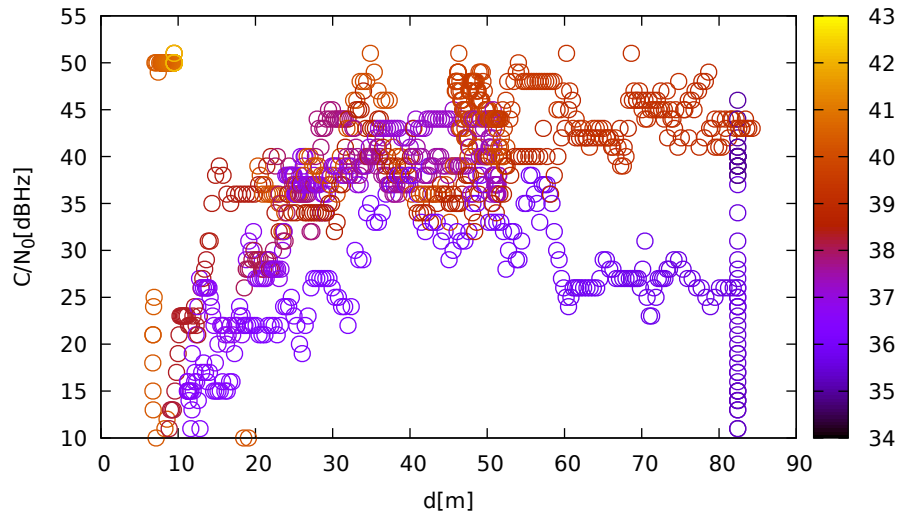
C/N 0 vs distance (ublox9 at C 3 for G32 at L1)
