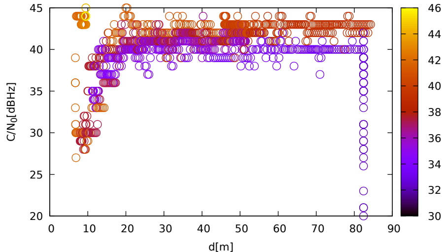
C/N 0 vs distance (ublox9 at C 3 for R06 at L1)
