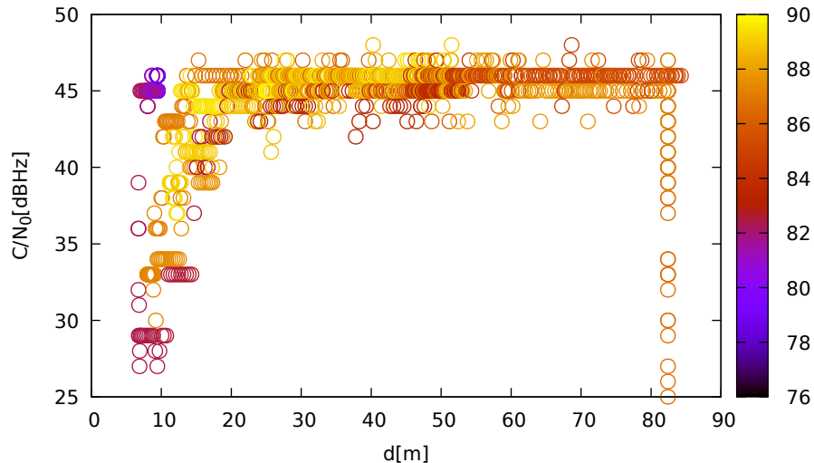
C/N_0 vs distance (ublox9 at C_3 for R07 at L1)
