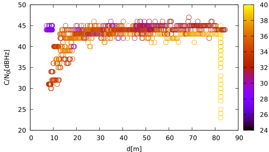
C/N_0 vs distance (ublox9 at C_3 for R08 at L1)
