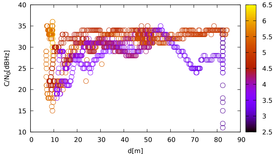
C/N_0 vs distance (ublox9 at C_3 for R14 at L1)
