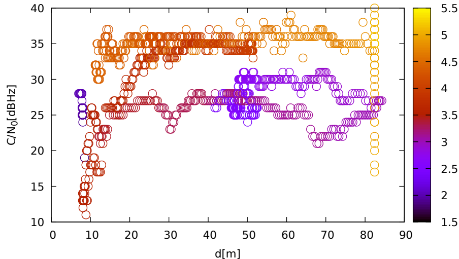
C/N 0 vs distance (ublox9 at C 3 for R15 at L1)
