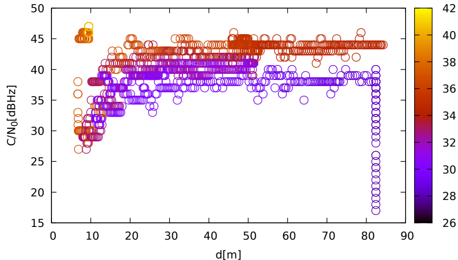
C/N_0 vs distance (ublox9 at C_3 for R21 at L1)
