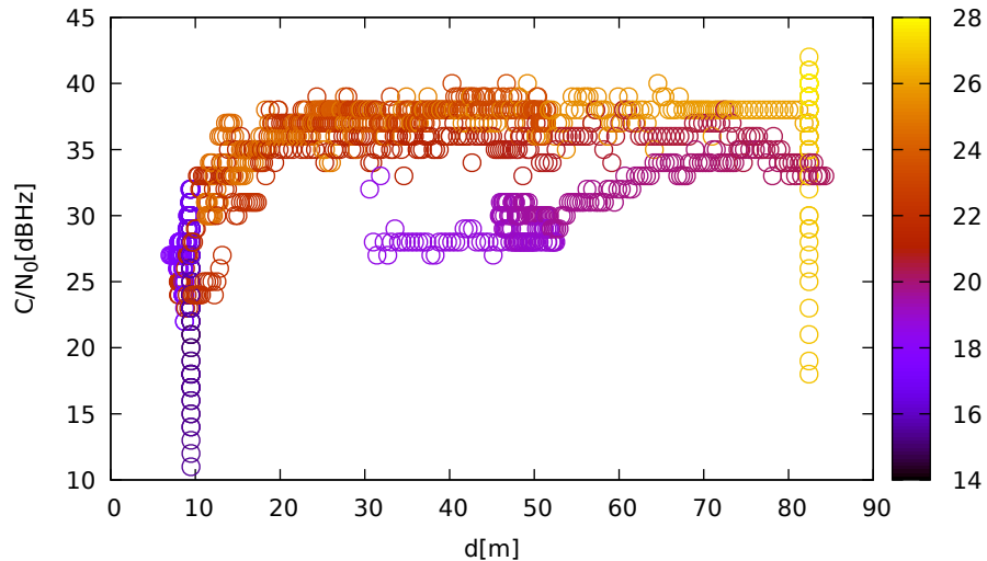
C/N 0 vs distance (ublox9 at C 3 for R23 at L1)
