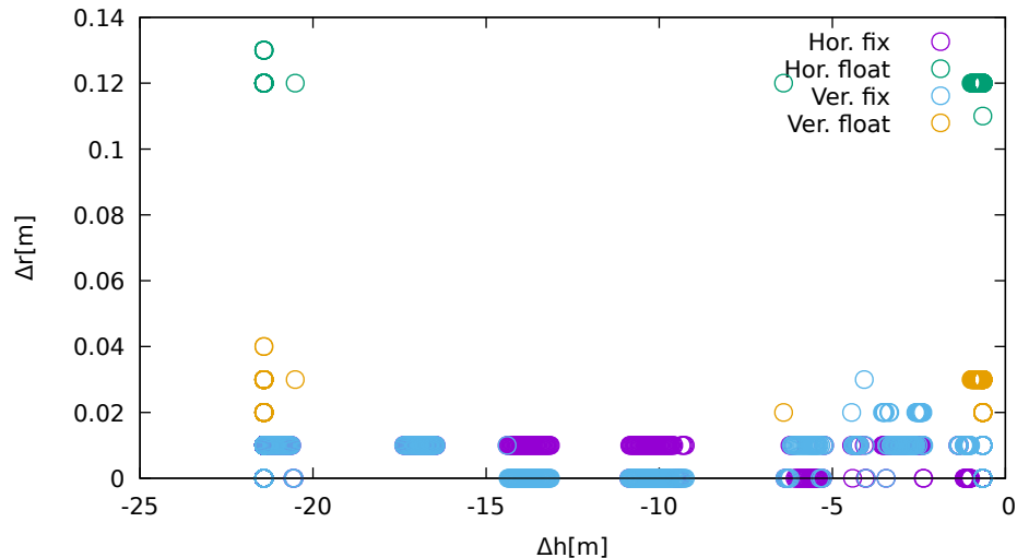
displacement vs distance (LeicaGS15 at down)
