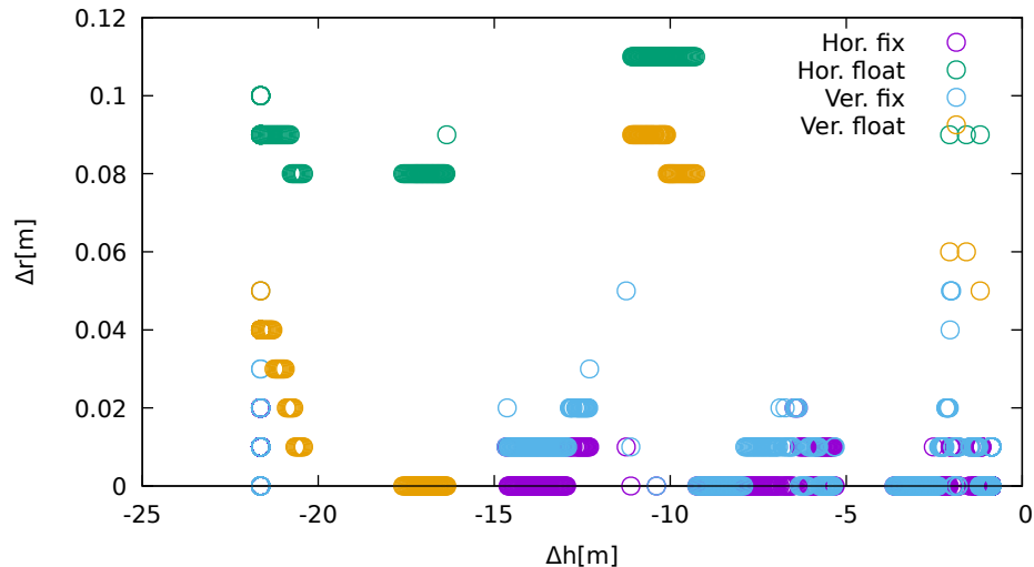
displacement vs distance (TrimbleR10 at down)
