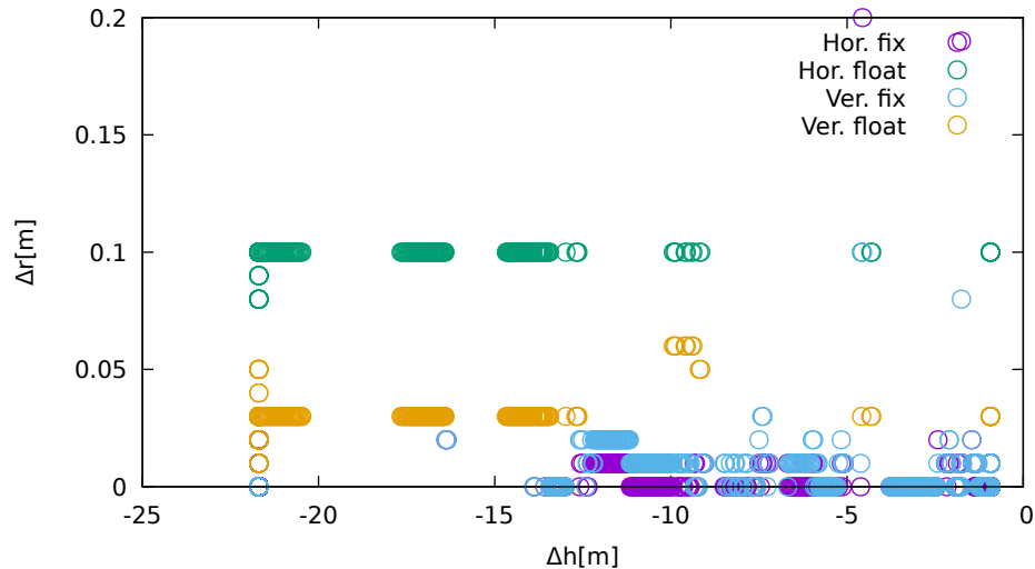
displacement vs distance (TrimbleR8s at down)
