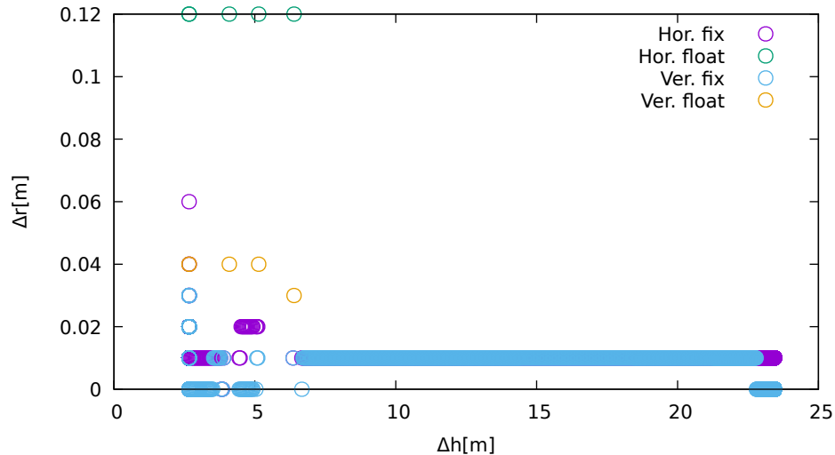
displacement vs distance (LeicaGS18 at up)
