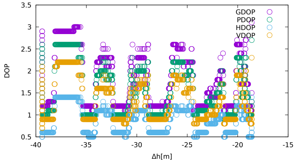
DOP vs height (JavadLSA - down)
