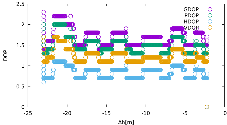
DOP vs height (JavadVS - down)
