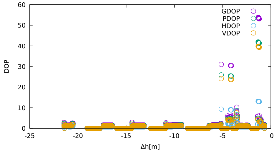
DOP vs height (LeicaGS15 - down)
