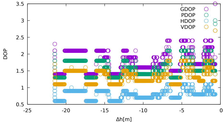
DOP vs height (LeicaGS18 - down)
