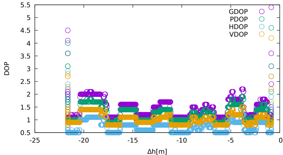
DOP vs height (TrimbleR10 - down)
