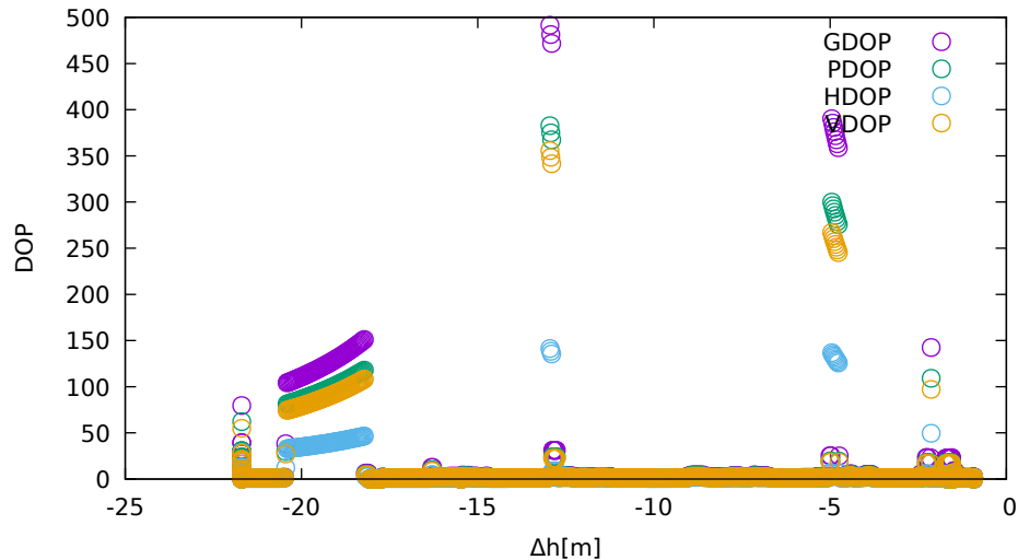
DOP vs height (TrimbleR8s - down)
