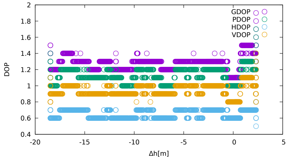
DOP vs height (ublox9 - down)
