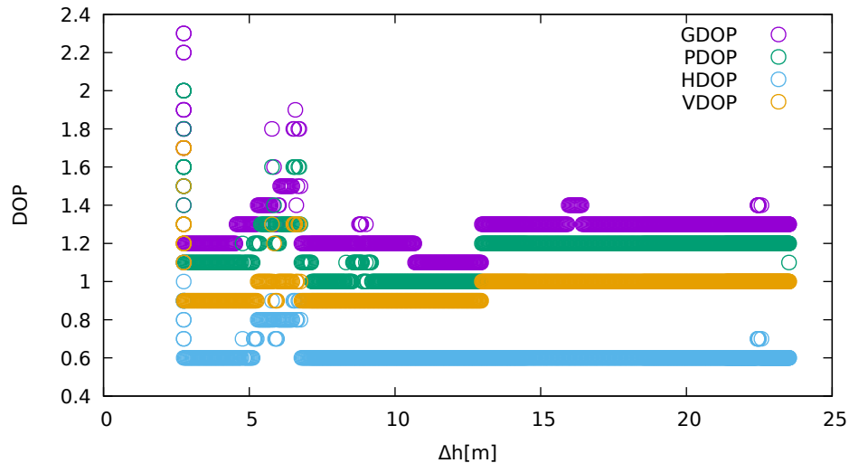
DOP vs height (JavadLSA - up)
