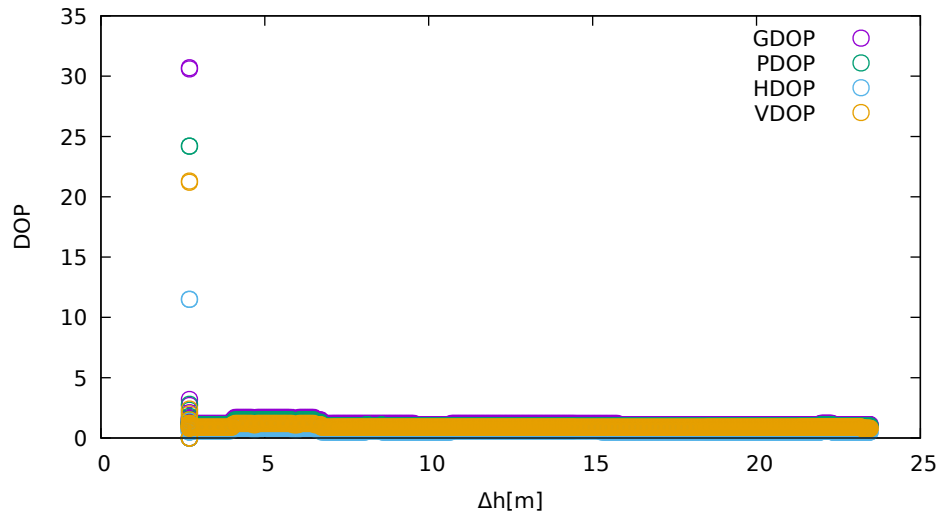
DOP vs height (LeicaGS15 - up)
