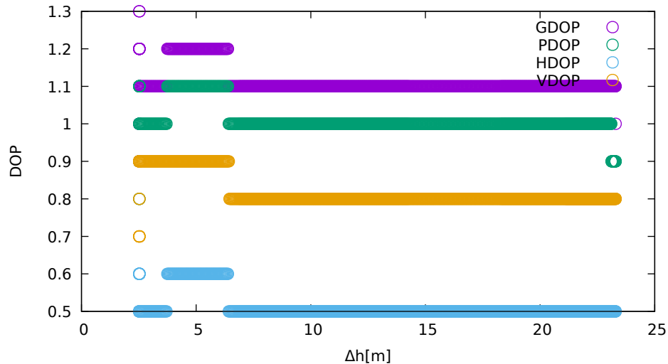
DOP vs height (ublox9 - up)
