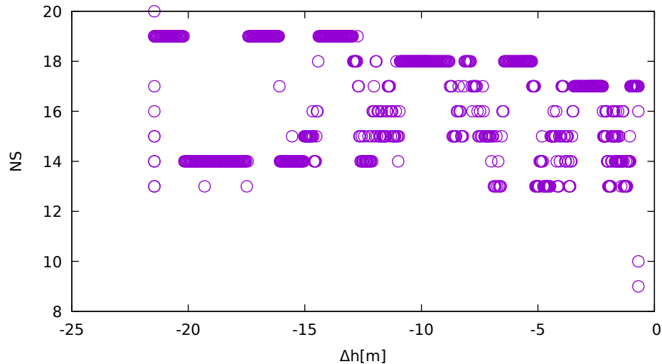
No. of satellites vs height (LeicaGS18 - down)
