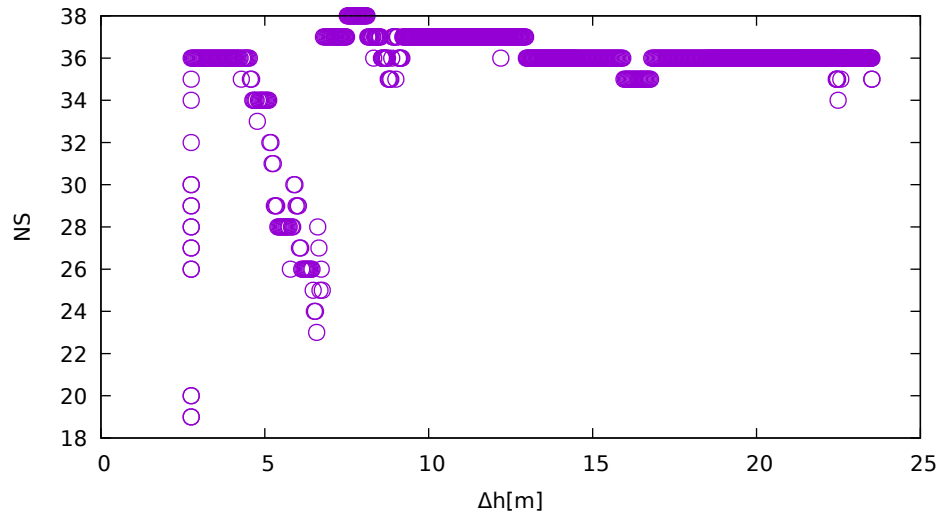
No. of satellites vs height (JavadLSA - up)
