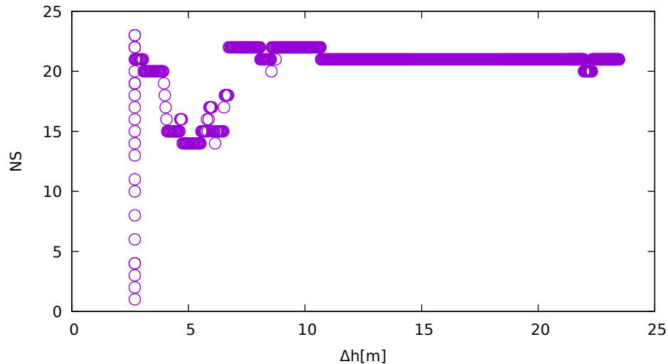
No. of satellites vs height (LeicaGS15 - up)
