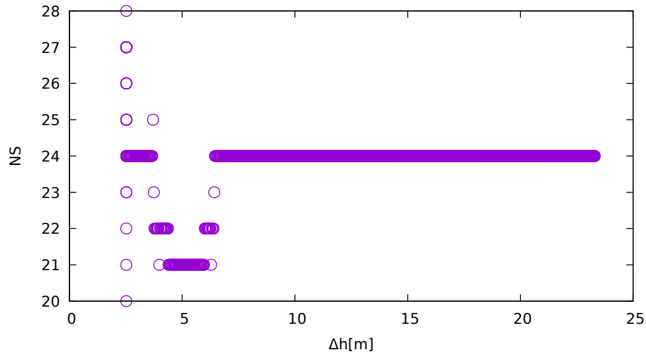
No. of satellites vs height (ublox9 - up)
