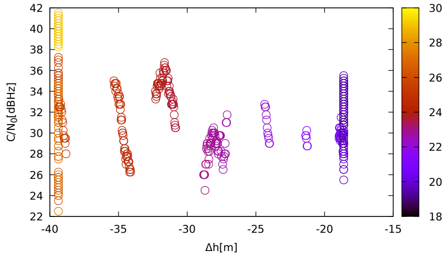
C/N 0 vs height (JavadLSA (down) for G16 at L1)
