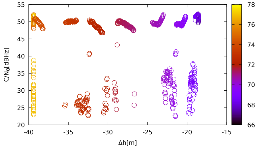
C/N 0 vs height (JavadLSA (down) for G18 at L1)
