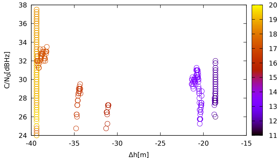
C/N 0 vs height (JavadLSA (down) for G20 at L1)
