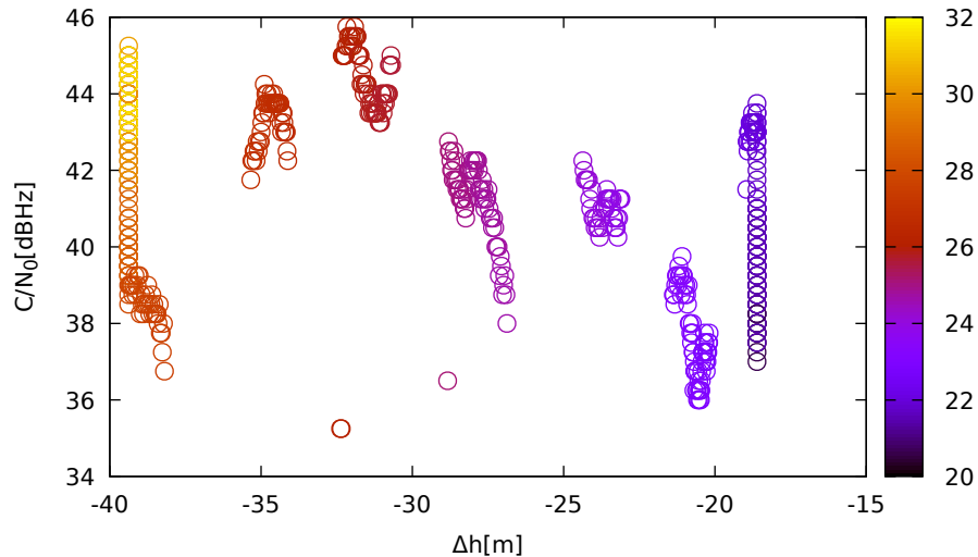
C/N 0 vs height (JavadLSA (down) for G21 at L1)
