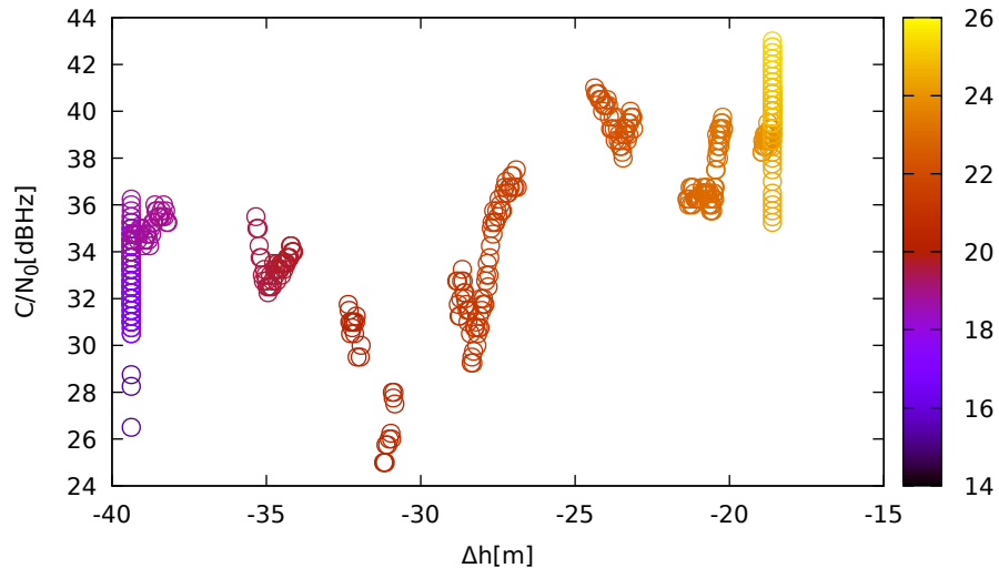
C/N 0 vs height (JavadLSA (down) for G25 at L1)
