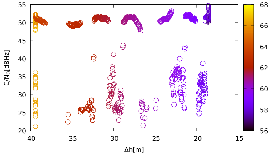
C/N 0 vs height (JavadLSA (down) for G26 at L1)
