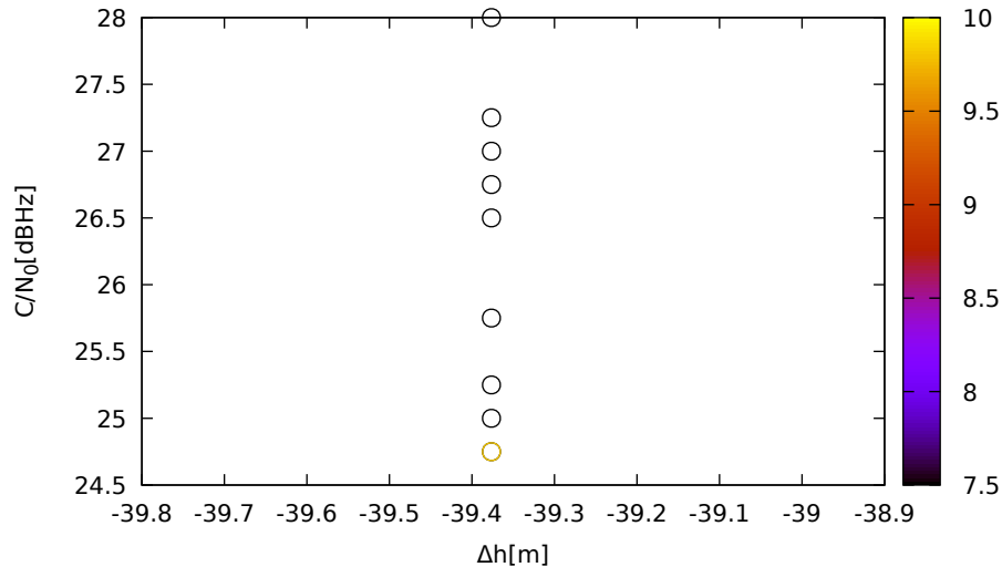
C/N 0 vs height (JavadLSA (down) for G27 at L1)
