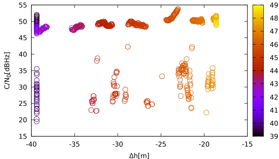
C/N 0 vs height (JavadLSA (down) for G29 at L1)
