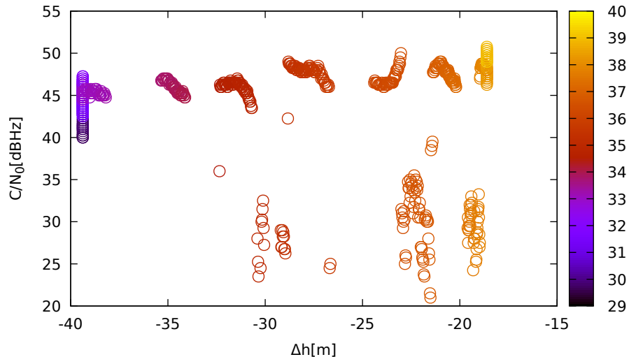
C/N 0 vs height (JavadLSA (down) for G31 at L1)
