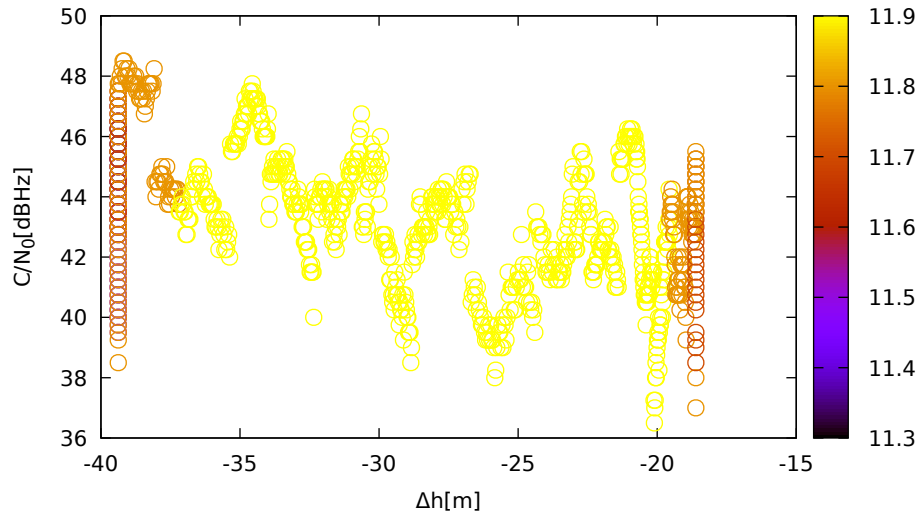
C/N 0 vs height (JavadLSA (down) for R02 at L1)
