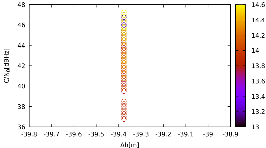
C/N 0 vs height (JavadLSA (down) for R03 at L1)
