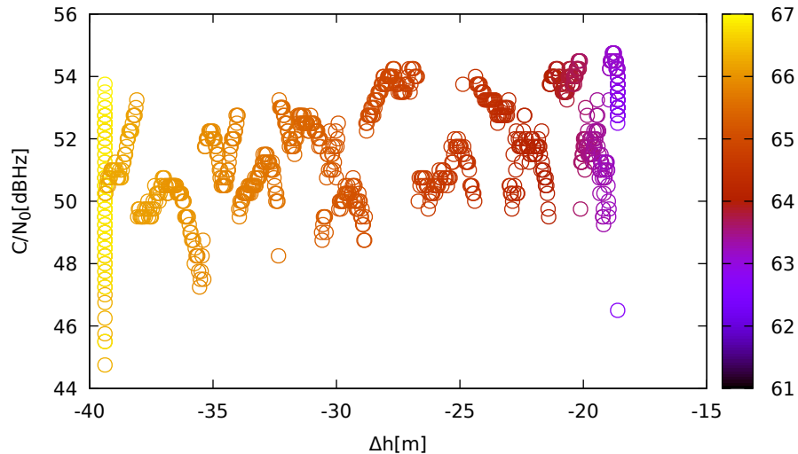
C/N 0 vs height (JavadLSA (down) for R09 at L1)
