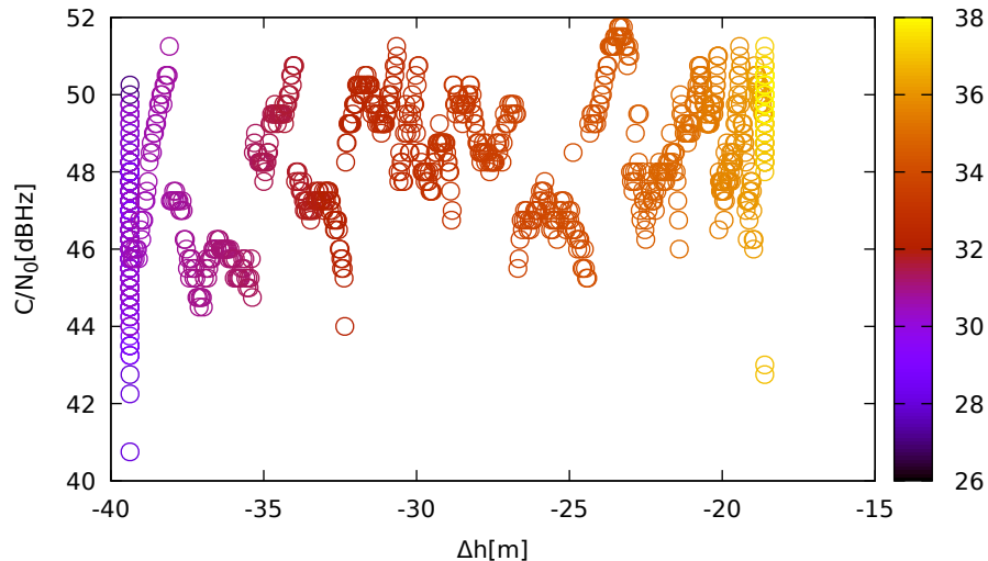
C/N 0 vs height (JavadLSA (down) for R18 at L1)
