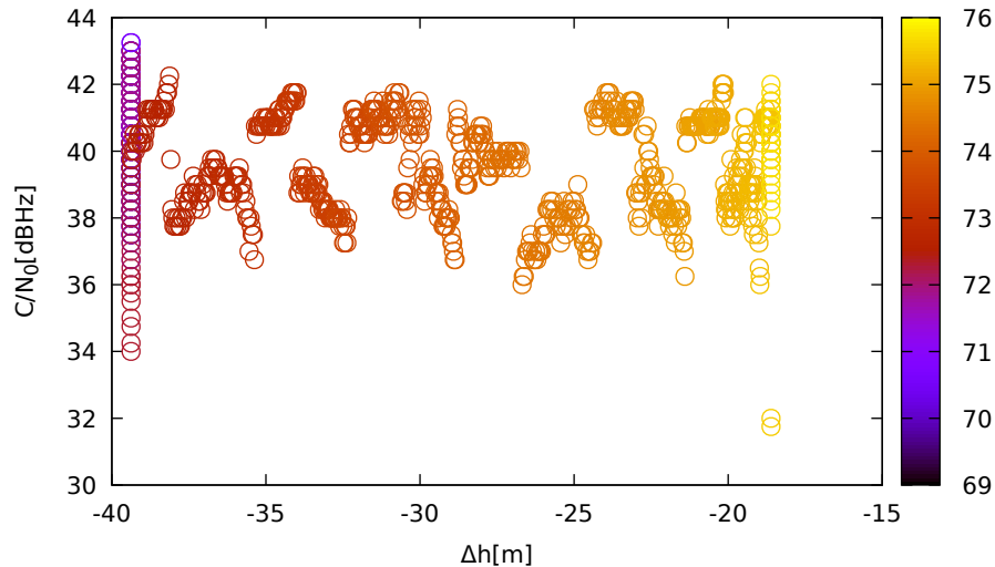
C/N 0 vs height (JavadLSA (down) for R19 at L1)
