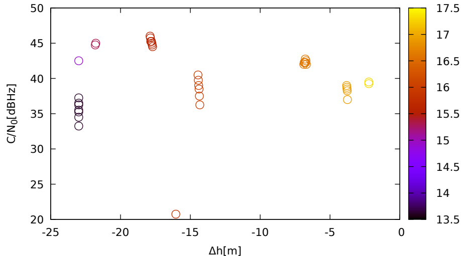
C/N 0 vs height (JavadVS (down) for G05 at L1)
