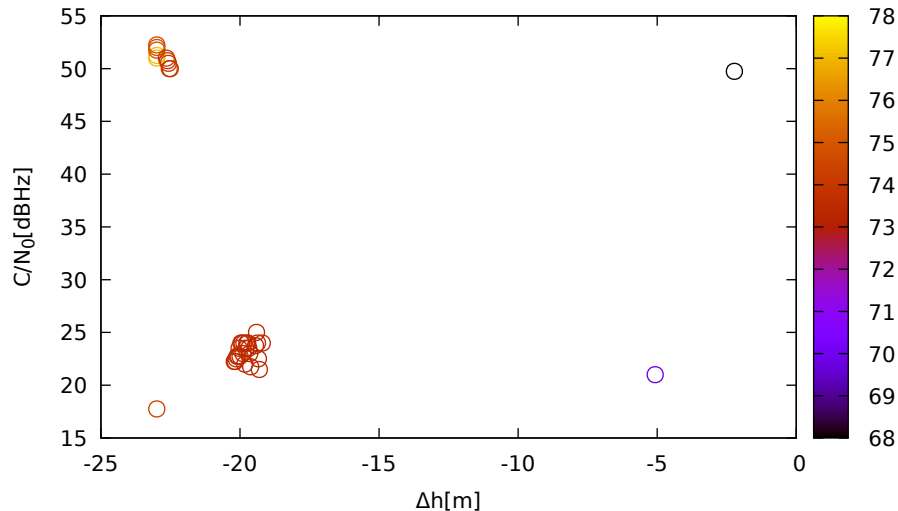
C/N 0 vs height (JavadVS (down) for G18 at L1)
