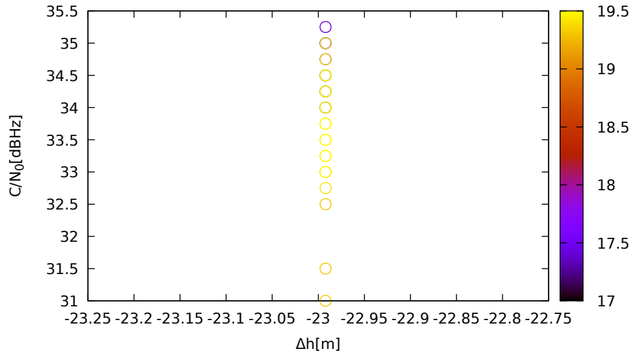
C/N 0 vs height (JavadVS (down) for G20 at L1)
