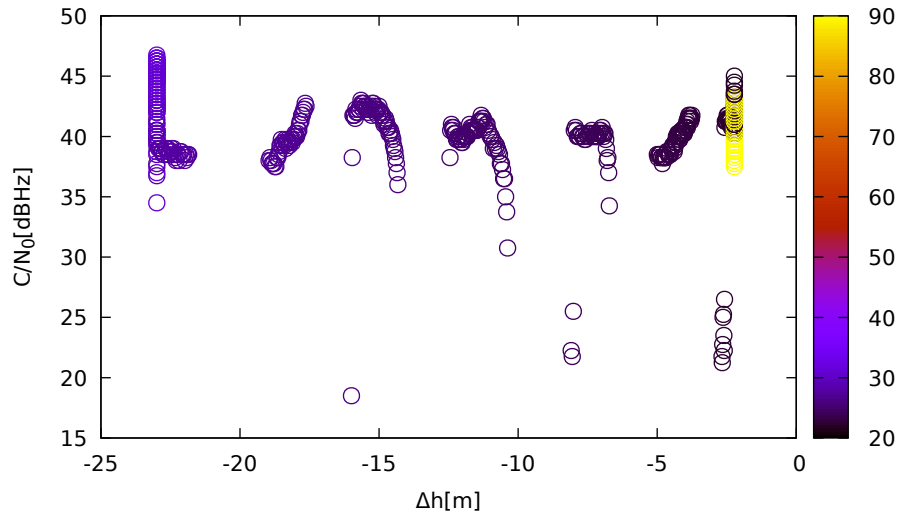
C/N 0 vs height (JavadVS (down) for G21 at L1)
