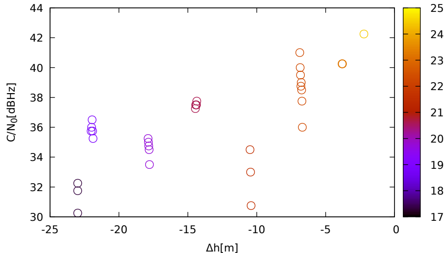
C/N 0 vs height (JavadVS (down) for G25 at L1)
