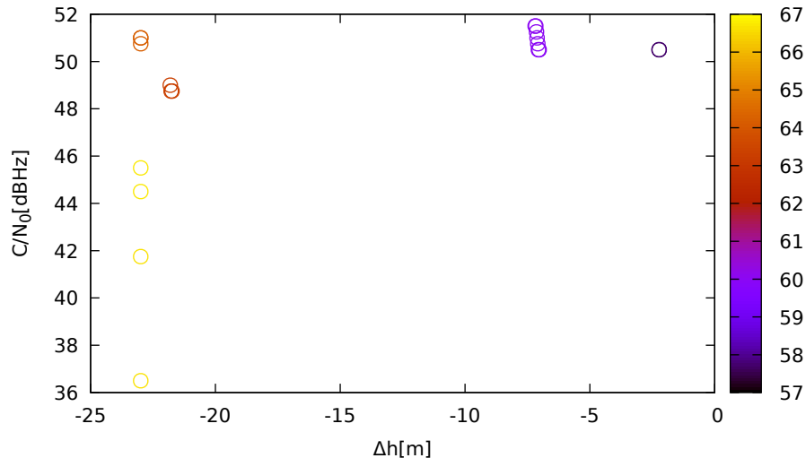
C/N 0 vs height (JavadVS (down) for G26 at L1)
