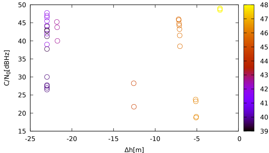
C/N 0 vs height (JavadVS (down) for G29 at L1)
