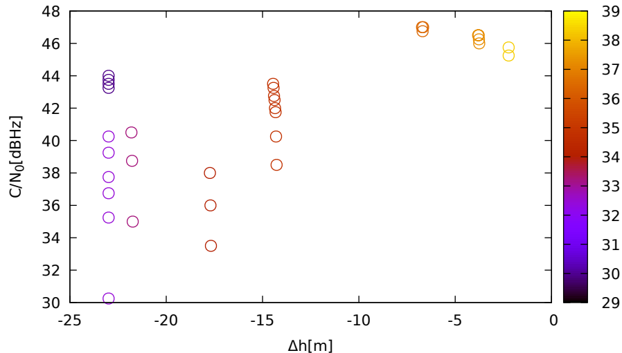
C/N 0 vs height (JavadVS (down) for G31 at L1)
