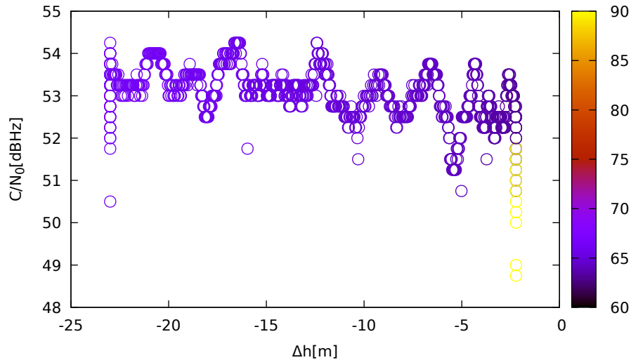
C/N 0 vs height (JavadVS (down) for R09 at L1)
