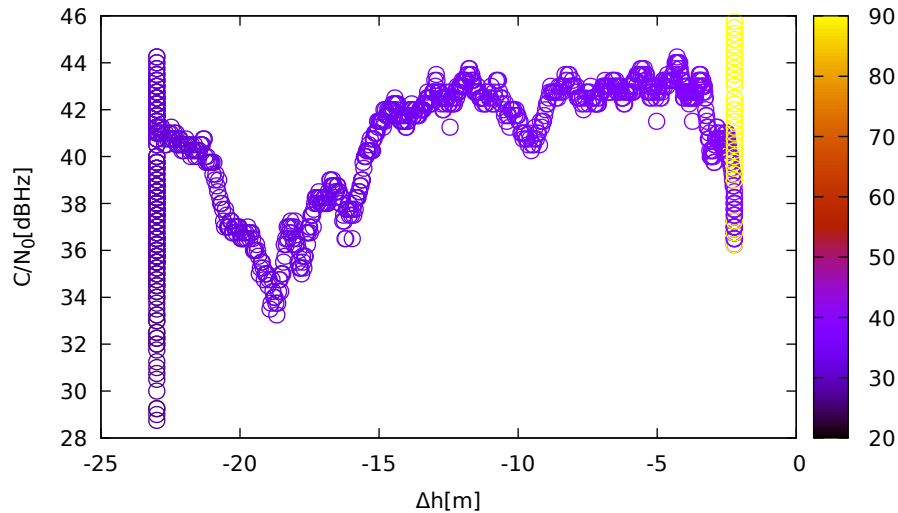
C/N 0 vs height (JavadVS (down) for R16 at L1)
